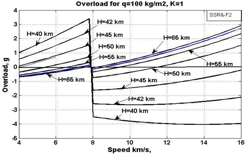
Fig. 6. Vertical overload via speed for the different altitudes, for ratio K = \text{Lift/drag} = \pm 1 and the special parachute load q = 100 \text{ kg/m}^2 . K = -1 for V > 8 \text{ km/s} .
