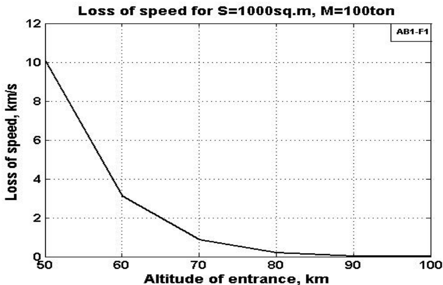
Fig.7. Loss of speed via altitude for distance L = 6378 \text{ km} (radius of the Earth) for mass of system 100 ton and parachute area 1000 \text{ m}^2 , q = 100 \text{ kg/sq.m.} .
