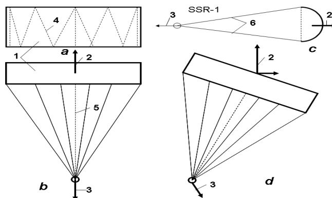
Fig.1. The offer design of a control high temperature parachute for braking space craft in the Earth high atmosphere. Notations: a –forward view (from space craft), b – side view, c –side view, d – creating of side force. 1 – parachute, 2 – brake force, 4 – 5 control cable (by changing the enter section), 6 – strops (cord, slings).
